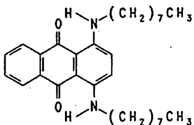
Compound 1a
